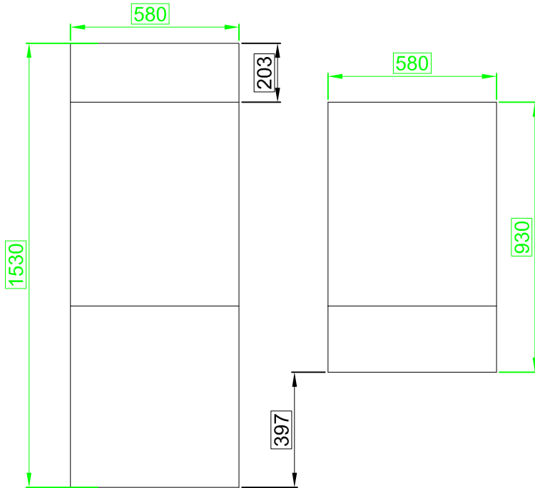
CHAIR MODULE Reclined position
